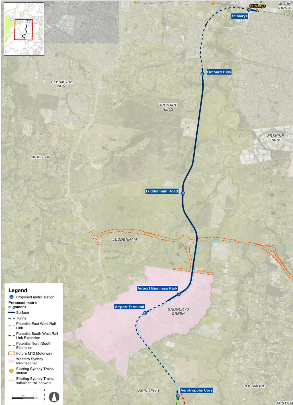
Figure 11 – First rail service alignment and potential alignment of second rail service
