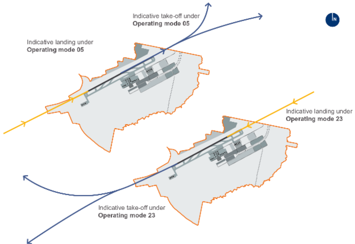
Figure 12: Arrival and departure modes for 05L and 23R 32
